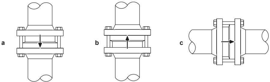
'b' is the only acceptable orientation when a DCV is supplied without an internal spring
